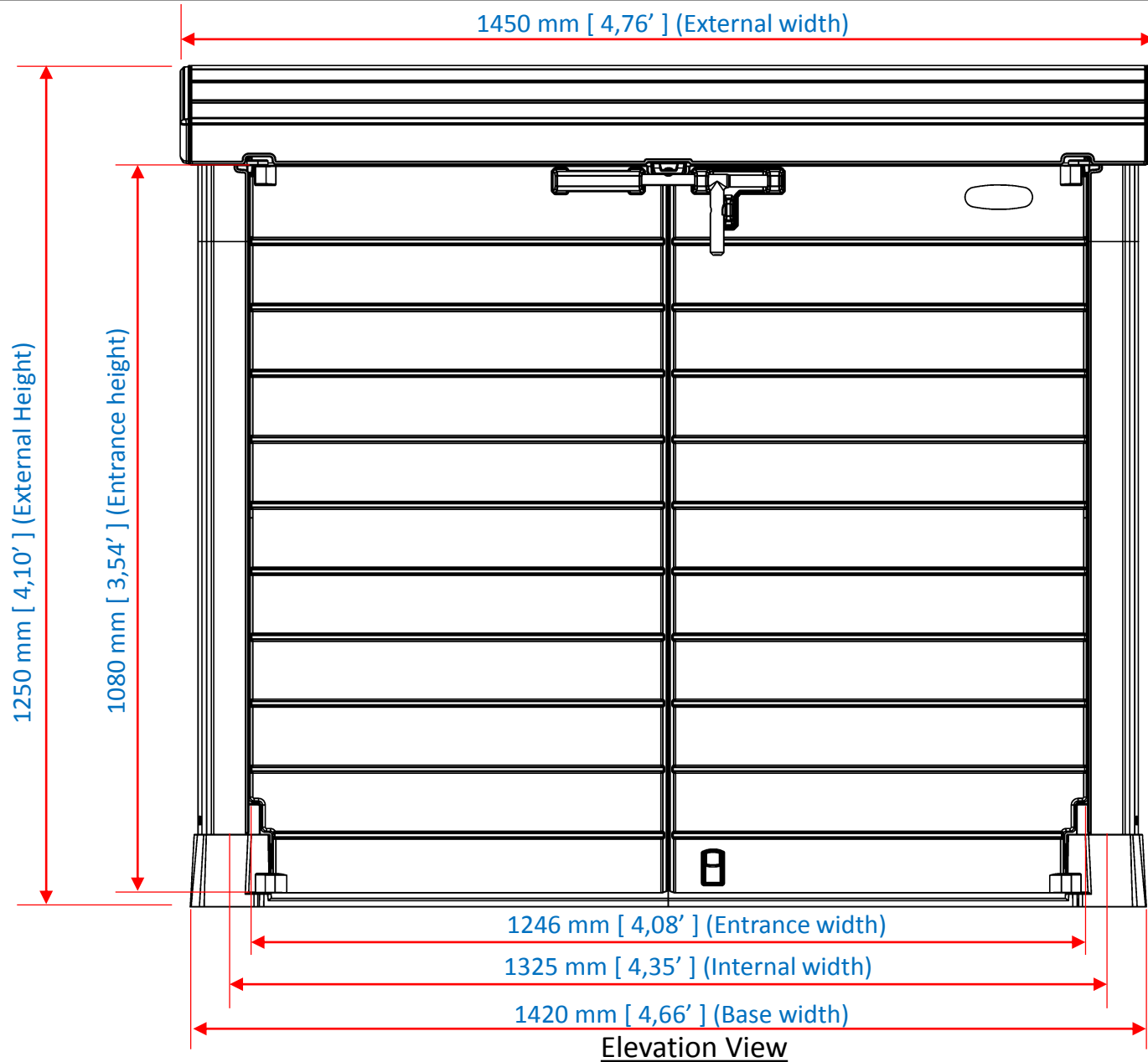
1200L Storage shed (Arc lid)
